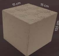
Bloco AF-2
