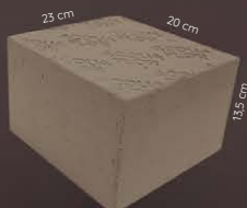
Bloco AF-4
